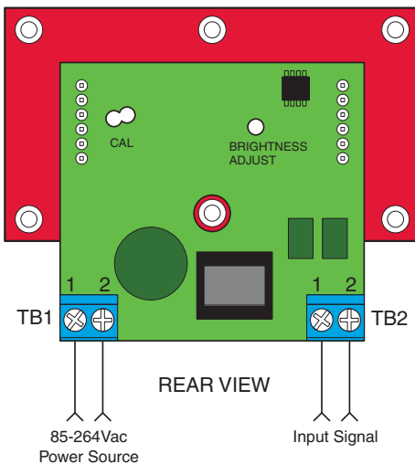
Figure 1. DMU-30DCV wiring diagram
